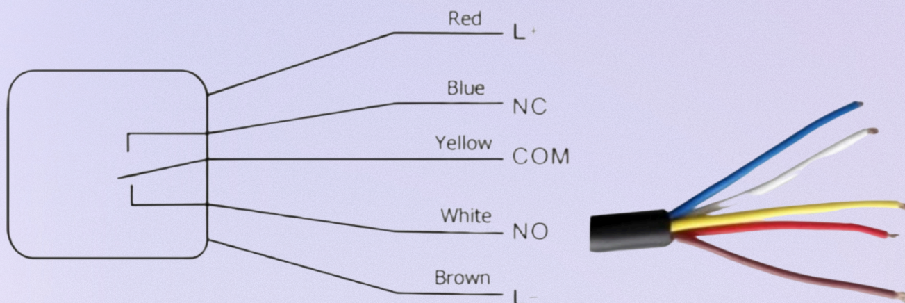
Wiring Diagram
